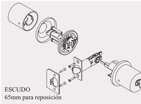
ROSETA 50mm
