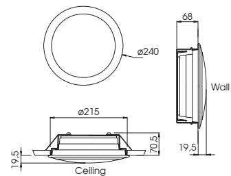
Hole required \varnothing 215 mm.
