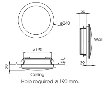
Hole required \varnothing 190 mm.
