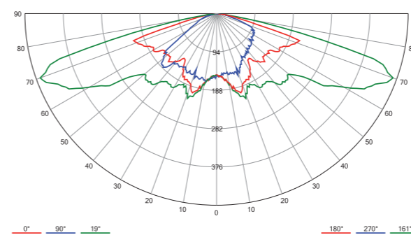
Reflector 1543 - SAP 70W
