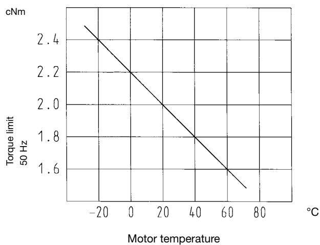
Chart: Torque limit versus motor temperature
