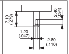
Quick-connect Z
