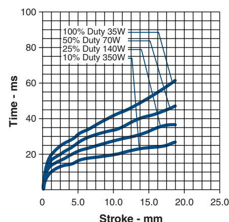
Size 7ECM— Typical Speed @ No Load, 20°C
