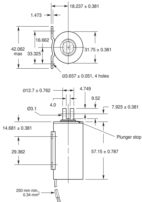
Ledex® Size 125M Pull — 32 mm Dia. x 57 mm
