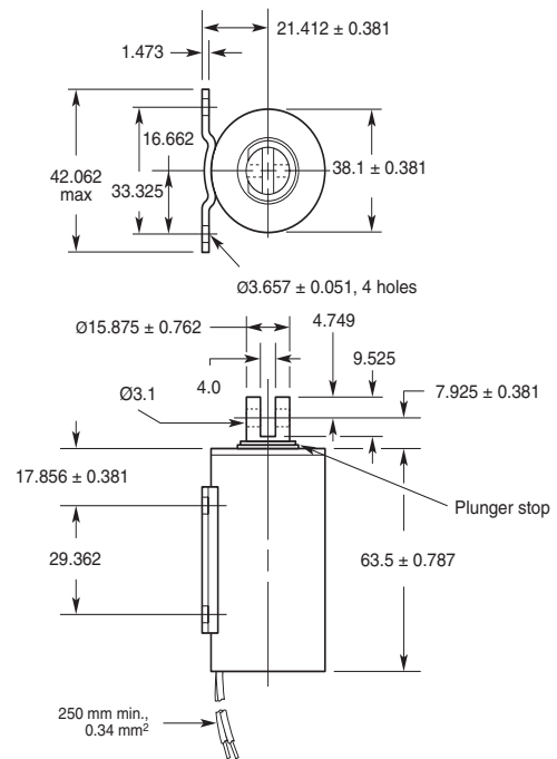
Ledex® Size 150M Pull — 38 mm Dia. x 64 mm
