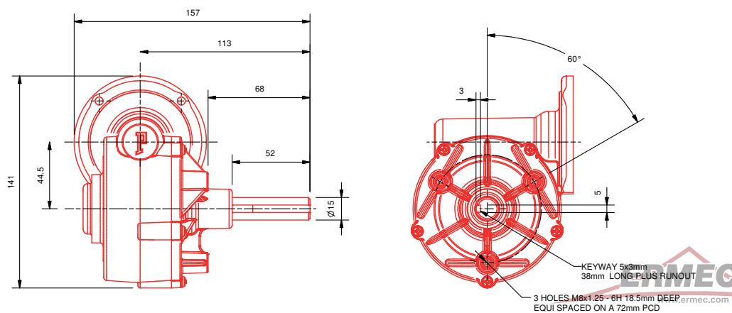
Parvalux L3P fixing option
