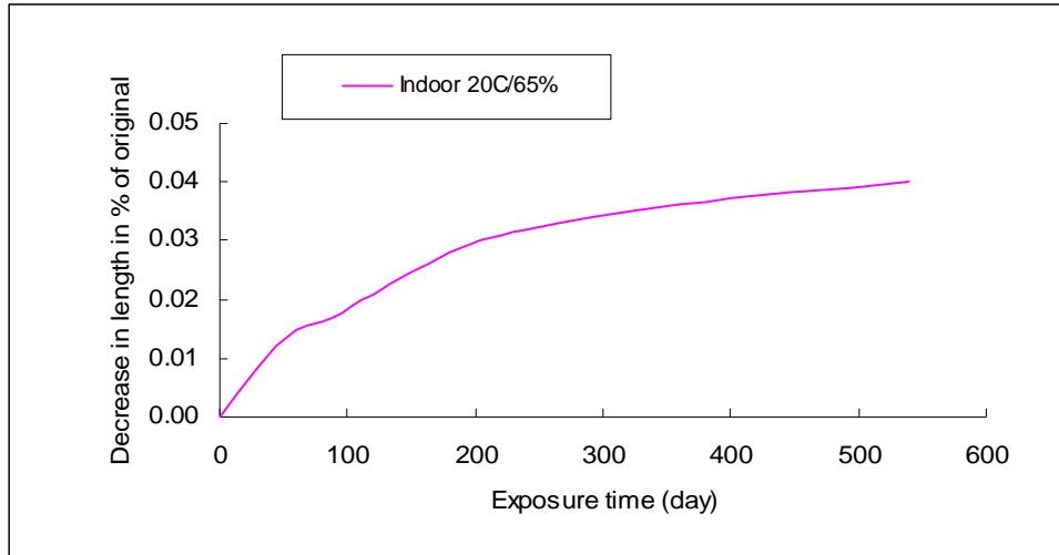
Figure 8 Average decrease in length of Viroc CBPB
