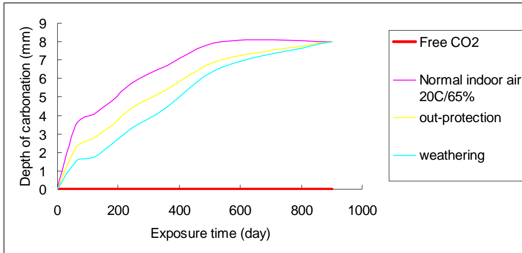
Figure 1 Mean depth of carbonation of Viroc CBPB with time under various exposure conditions
