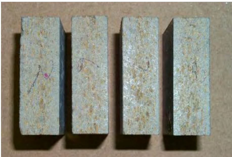
Figure 4 Fully carbonated Viroc CBPB after 2 year's exposure under normal indoor air environment
