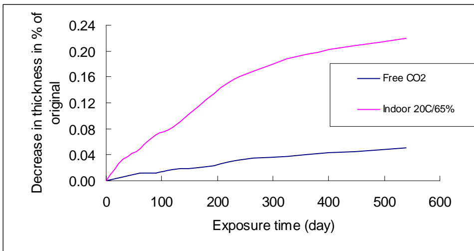
Figure 7 Average decrease in thickness of Viroc CBPB
