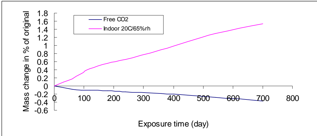
Figure 6 Average increase in mass of Viroc CBPB
