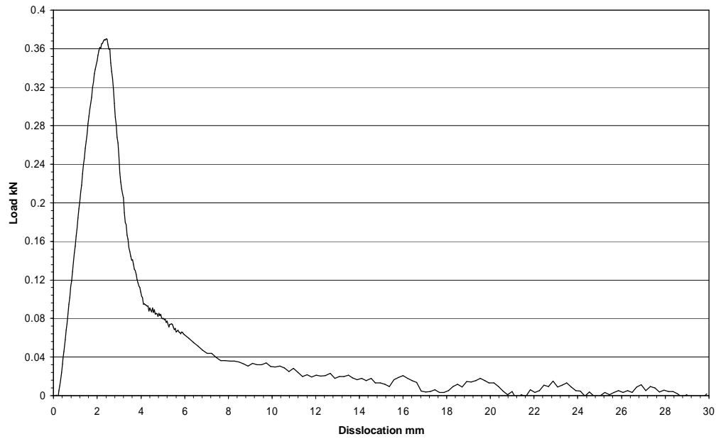
Figure B2 Stress-strain curve of Sample 135: Fmax=370.29N
