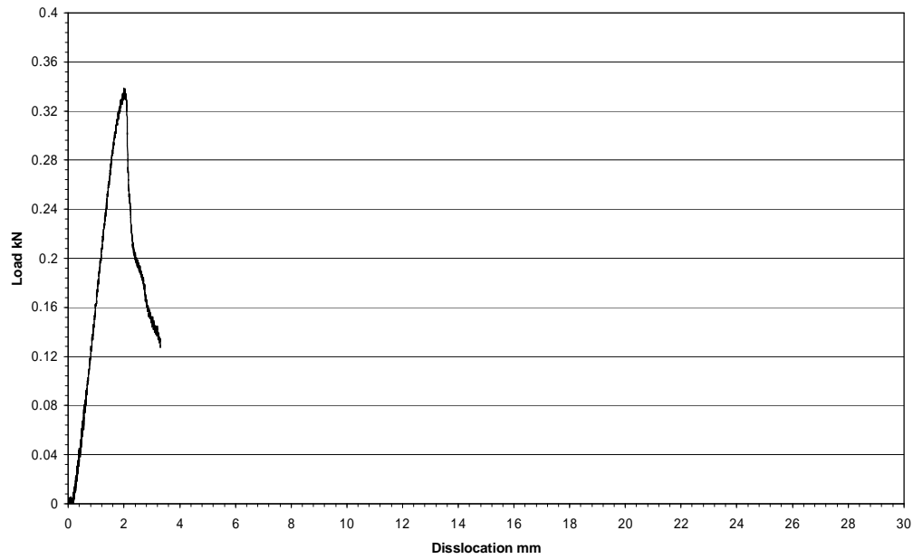
Figure B4 Stress-strain curve of Sample 189: Fmax=338.61N
