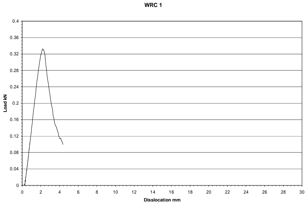
Figure B1 Stress-strain curve of Sample 123: Fmax=332.30N
