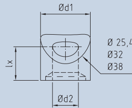
Angle washer for countersunk end stop 90°, round profile
